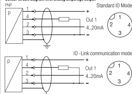
Sensor circuit diagram with analog amperage output
