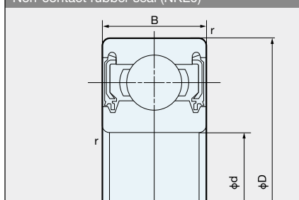
Non-contact rubber seal (NKE9)
