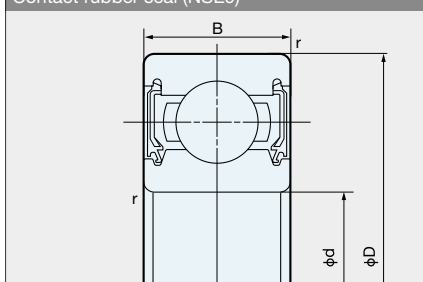
Contact rubber seal (NSE9)
