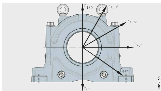
Figure 19 Load directions F for the guide values for the housing rupture load and the maximum load carrying capacity of the connecting screws
