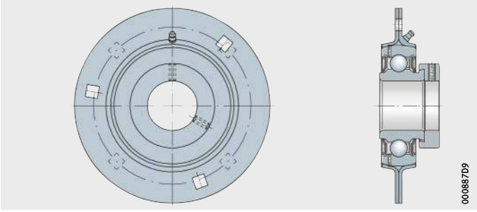
Figure 6 Flanged bearing unit with sheet steel housing
