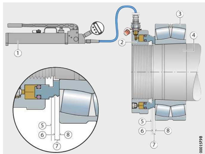
Figure 3 Mounting of a spherical roller bearing using PUMP1000-4L-CONTROL
