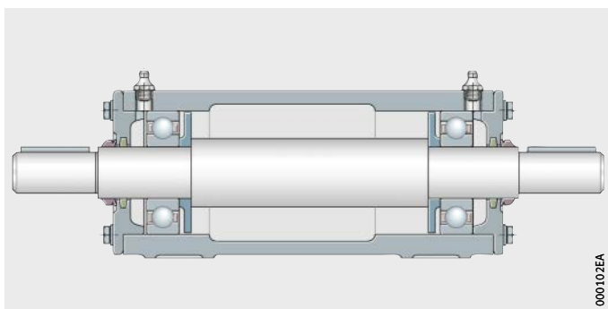
Figure 2 Plummer block housing unit VRE3...-A
