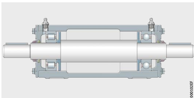
Figure 3 Plummer block housing unit VRE3...-B
