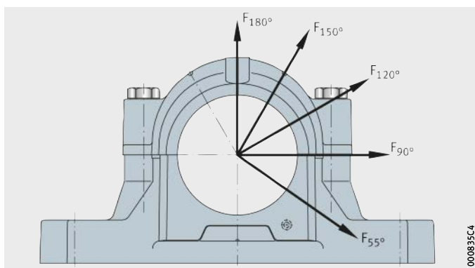
Figure 10 Load directions F for the guide values for the housing rupture load and the maximum load carrying capacity of the connecting screws
